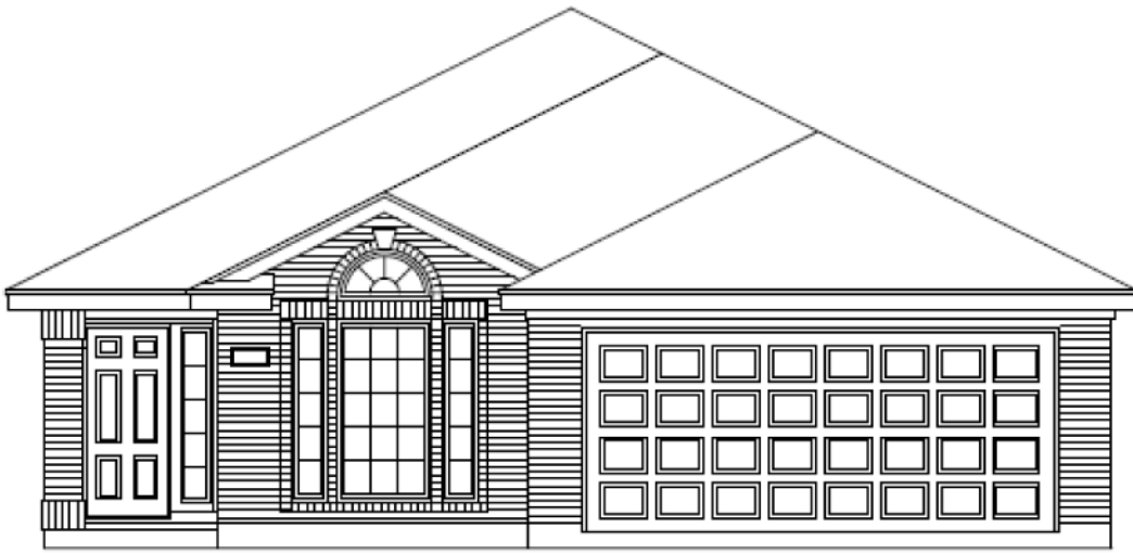
Elevation "B"
