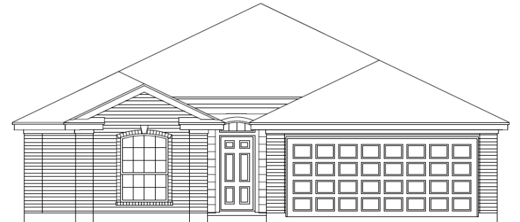
ELEVATION "A"
