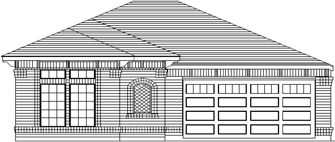
Elevation "A"
