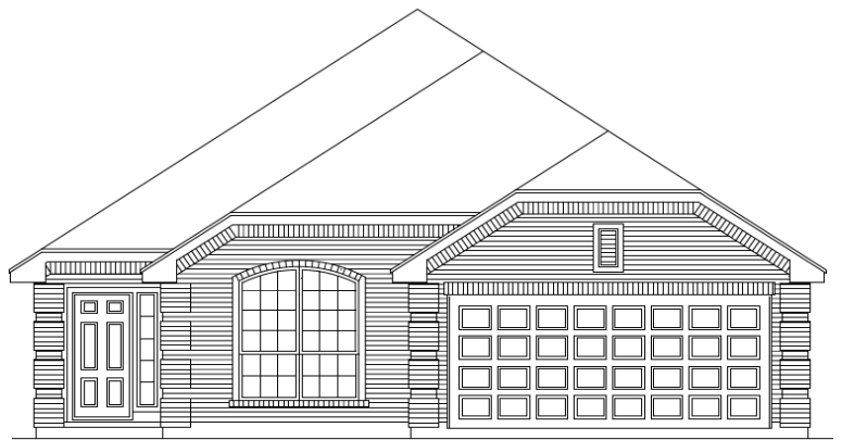
Elevation "E"
